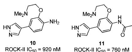
Figure 2. Compounds 10 and 11 and their ROCK-II potency.
